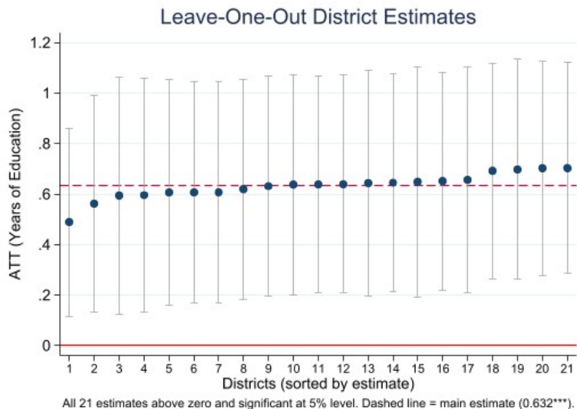
Figure 9: Leave-One-Out Robustness
