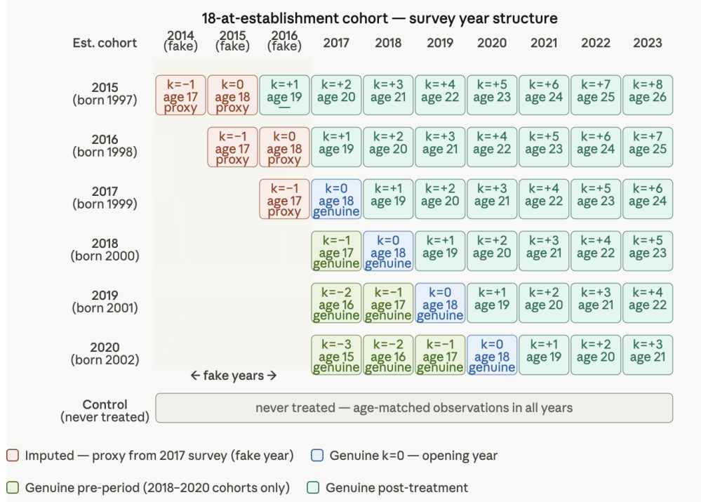
Figure 10: Sample Construction
