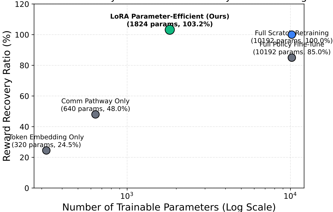
Parameter Efficiency: Performance Recovery vs. Tuned Weights
