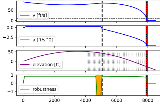
(c) Base enforcement algorithm [24] without offset overshoots by 14ft \zeta . Light-gray dotted lines mark other movement authority endpoints in the range 4000ft–8000ft that the algorithm would also overshoot.
