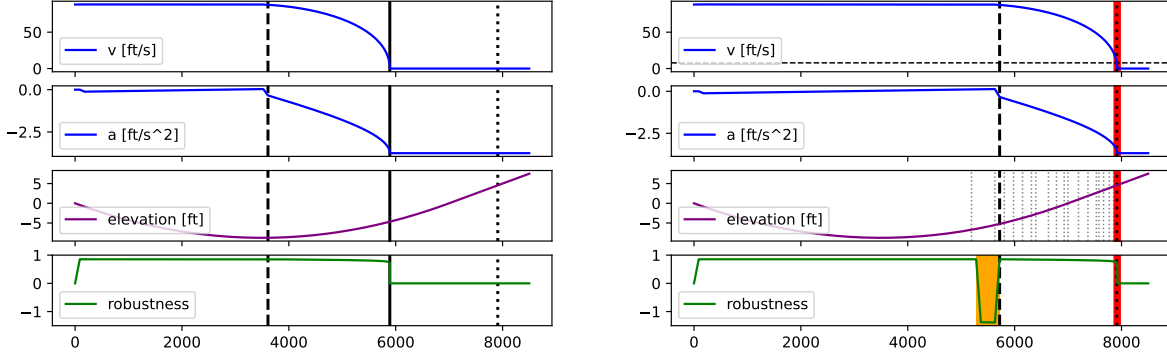
(a) Base enforcement algorithm [24] initiates braking at 3609ft and stops at position 5889ft with an undershoot of 2021ft, which exceeds the 1000ft maximum undershoot performance objective [24]. (b) Base enforcement algorithm [24] without offset overshoots by 9ft. Light-gray dotted lines mark other challenging movement authority endpoints in the range 4000ft–8000ft that would also be violated.
