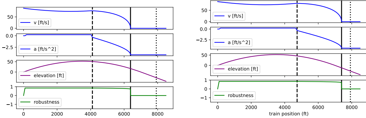
(a) Base enforcement algorithm [27] undershoots by 1539ft. (b) Verified control envelope (Model 5) limits undershoot to 528ft.
