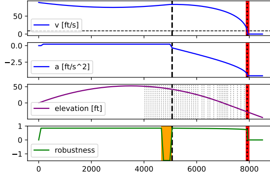
(c) Base enforcement algorithm [27] without offset overshoots by 14ft \nabla . Light-gray dotted lines mark other movement authority endpoints in the range 4000ft–8000ft that the algorithm would also overshoot.
