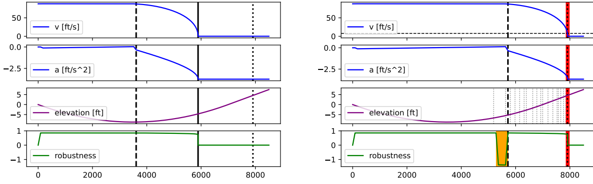
(a) Base enforcement algorithm [27] initiates braking at 3609ft and stops at position 5889ft with an undershoot of 2021ft, which exceeds the 1000ft maximum undershoot performance objective [27]. (b) Base enforcement algorithm [27] without offset overshoots by 9ft. Light-gray dotted lines mark other challenging movement authority endpoints in the range 4000ft–8000ft that would also be violated.
