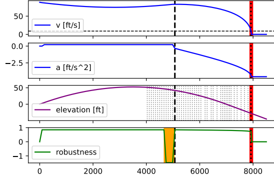
(c) Base enforcement algorithm [24] without offset overshoots by 14ft \nabla . Light-gray dotted lines mark other movement authority endpoints in the range 4000ft–8000ft that the algorithm would also overshoot.
