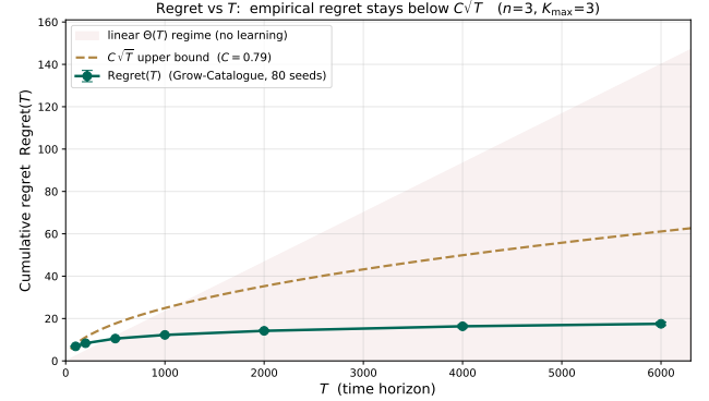
Figure 3: Cumulative regret versus horizon T for GROW-CATALOGUE ( n = 3 , K_{\max} = 3 , uniform random adversary, 80 seeds). The green curve stays strictly below the C\sqrt{T} upper envelope implied by Theorem 6, which is in turn well below the linear-regret regime that would result without learning.
