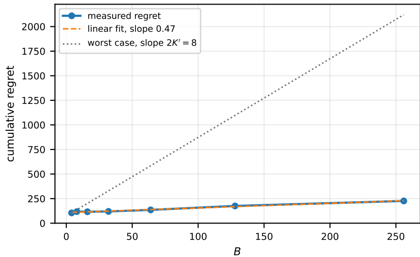
(c) n = 10 : regret versus revelation granularity B
