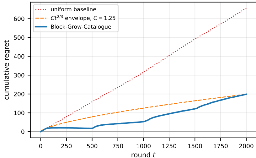
(b) n = 20, K_{\max} = 4, B = 40
