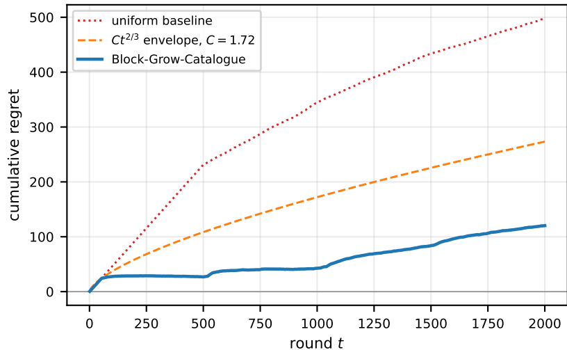
(a) n = 10, K_{\max} = 4, B = 40
