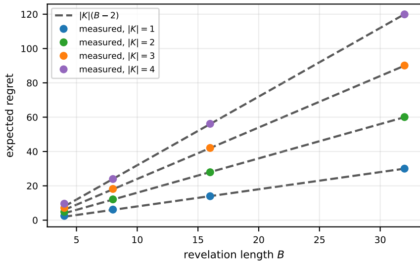
(c) scheduled revelation: \text{regret} \geq |K|(B - 2) (Thm. 22)
