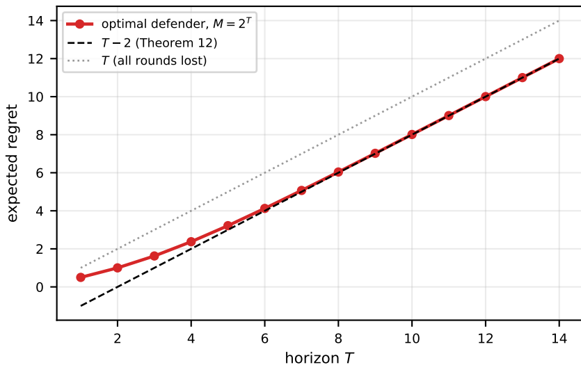
(a) infinite universe: \mathbb{E}[\text{Regret}] = T - 2 + o(1)
