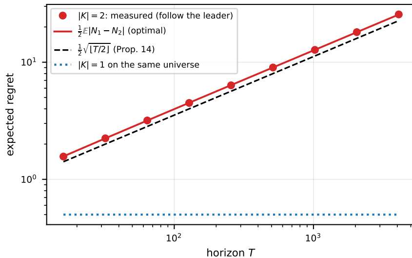
(b) two types already cost \sqrt{T} , at |\mathcal{U}| = 2
