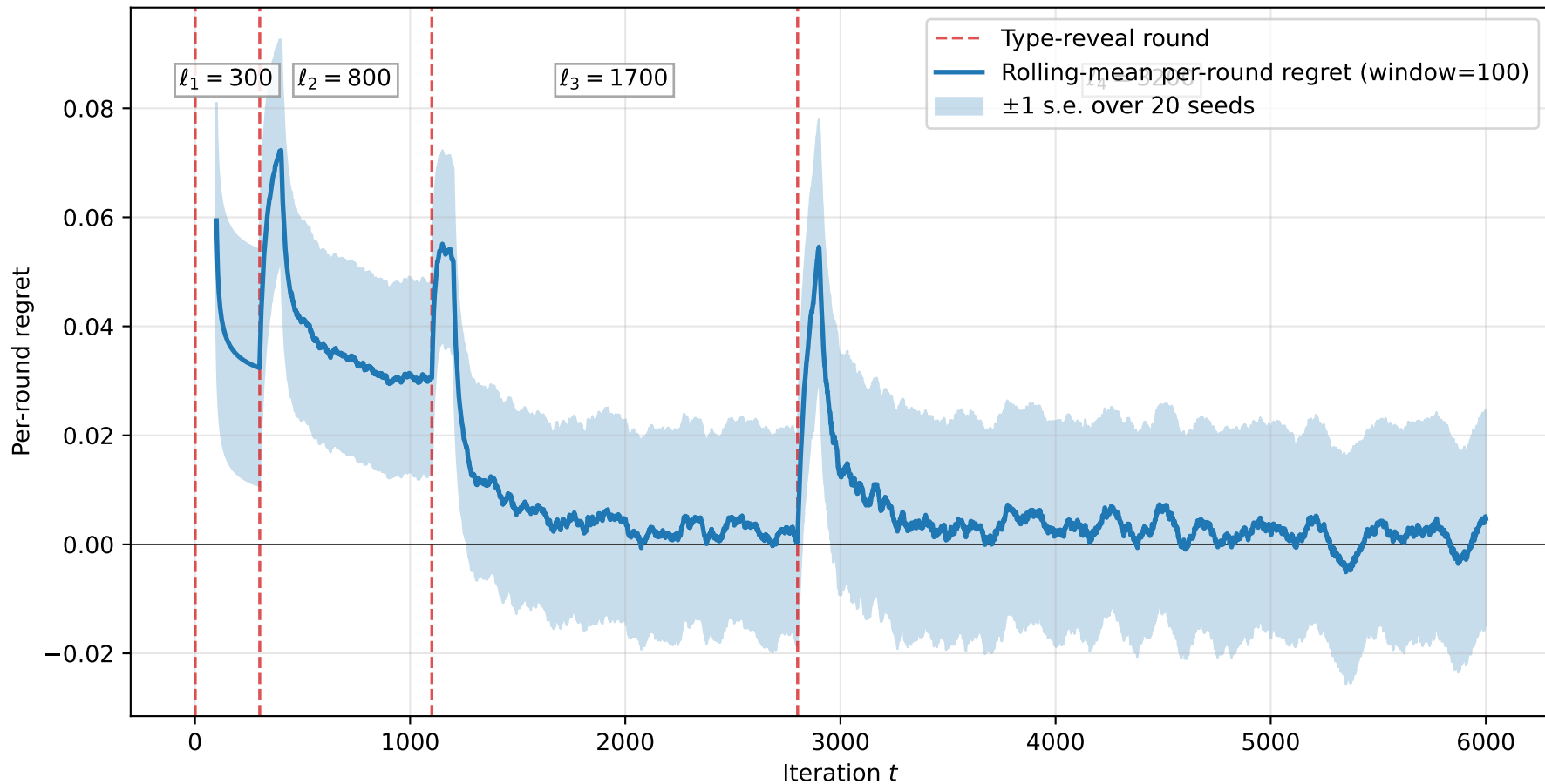
GROW-CATALOGUE on non-uniform epochs ( n = 5 , K_{\max} = 4 , \ell = [300, 800, 1700, 3200] , sampled \mathcal{E} )
