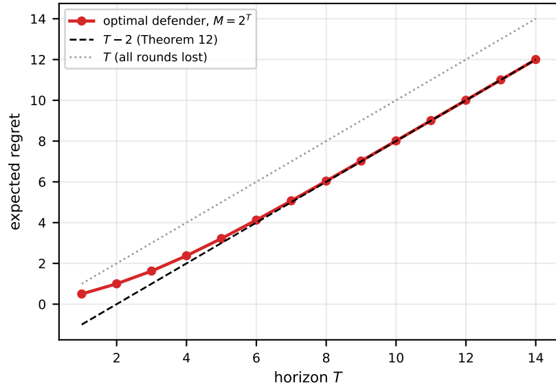
(a) infinite universe: \mathbb{E}[\text{Regret}] = T - 2 + o(1)
