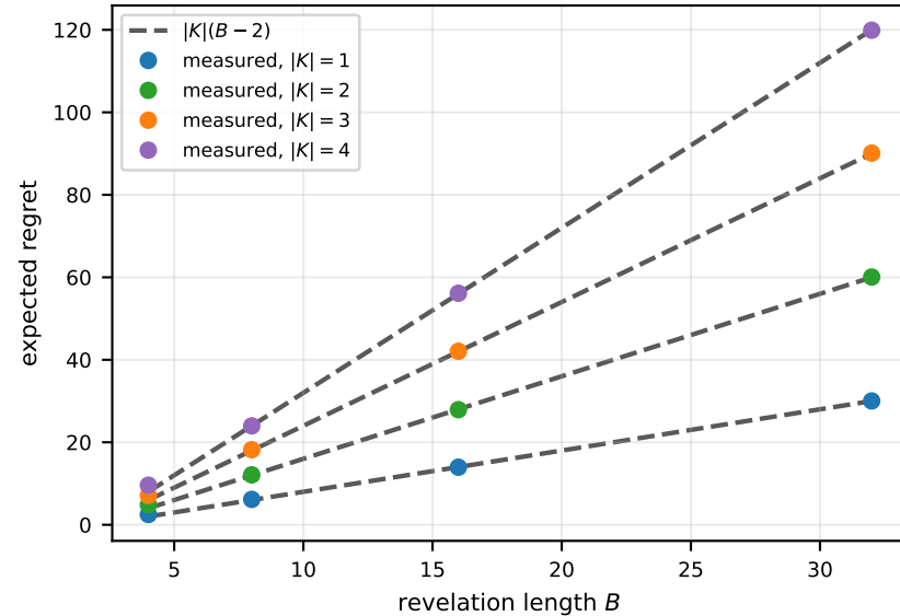
(c) scheduled revelation: regret \geq |K|(B - 2) (Thm. 22)
