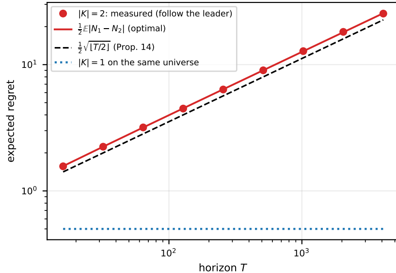
(b) two types already cost \sqrt{T} , at |\mathcal{U}| = 2
