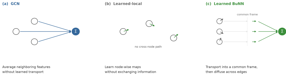
Figure 1: Schematic distinction among GCN aggregation, the learned-local capacity control, and learned bundle transport. The drawing describes a computational operation only; it does not represent biological signal flow.
