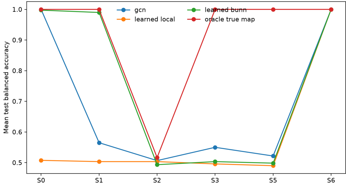
Figure 11: Mean test balanced accuracy across E2 conditions. S1 provides fixed recoverable geometry; S2, S3, and S5 break topology, marker assignment, and across-participant learnability. S6 supplies an already-global summary.
