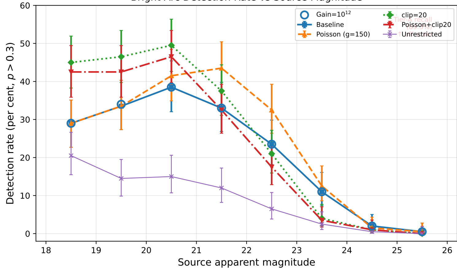
Bright-Arc Detection Rate vs Source Magnitude
