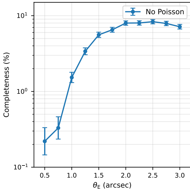
Completeness vs \theta_E ( p > 0.3 )
