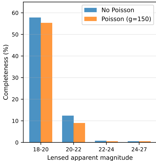
Completeness vs lensed mag ( p > 0.3 )
