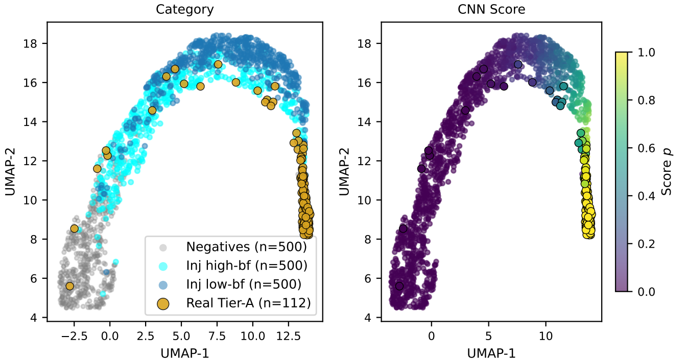
Figure 2. Two-panel UMAP projection of CNN penultimate-layer (1280-dimensional) embeddings. Left: Points coloured by category — real Tier-A (gold), low- \beta_{\text{frac}} injections (blue), high- \beta_{\text{frac}} injections (cyan), negatives (grey). Right: Same projection coloured by CNN score ( p , continuous colourbar from 0 to 1). UMAP computed with n_neighbors=30 , min_dist=0.3 , metric=cosine , random_state=42 . Colourbar: viridis (right panel).
