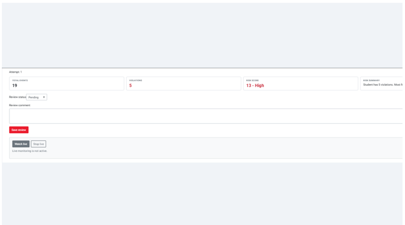
Gambar 8: Form review
