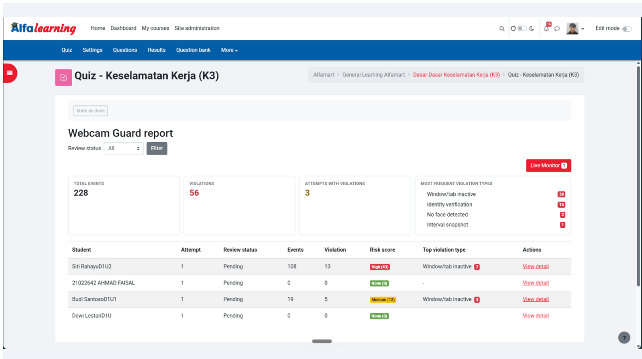
Gambar 6: Halaman report
