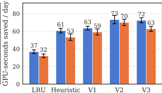
(b) Delivered value: LRU loses both
