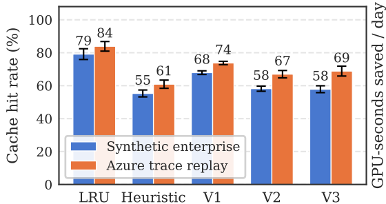
(a) Hit rate: LRU wins both
