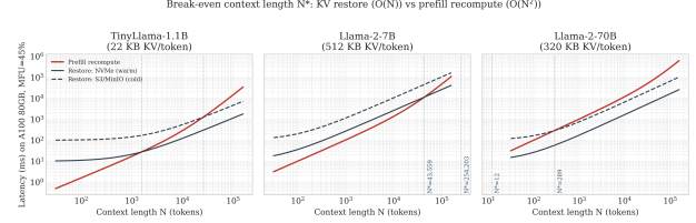
Figure 5: Prefill recompute ( O(N^2) , red) vs. tier restore ( O(N) , black) latency by context length. The crossover N^* varies by four orders of magnitude across model architectures.
