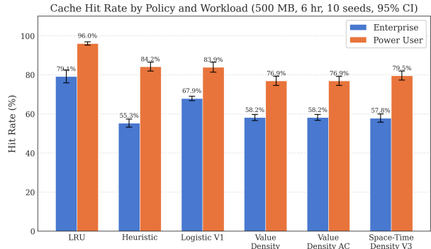
Figure 1: Cache hit rate by policy and workload, 95% CIs across 10 seeds. LRU wins this metric on both constrained workloads; Figure 2 shows what that does not imply.
