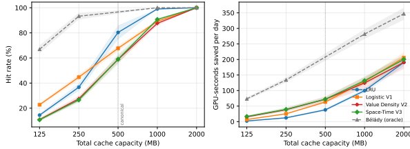
Figure 4: Capacity sweep (enterprise, 5 paired seeds, shaded 95% CIs). Left: hit rate converges to 100% for every policy as capacity grows. Right: delivered value does not converge. The dotted line marks the canonical 500 MB operating point.
