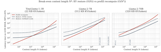
Figure 5: Prefill recompute ( O(N^2) , red) vs. tier restore ( O(N) , black) latency by context length. The crossover N^* varies by four orders of magnitude across model architectures.
