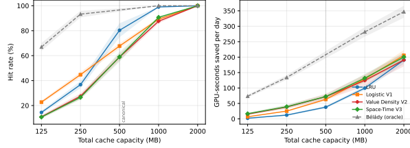
Figure 3: Capacity sweep (enterprise, 5 paired seeds, shaded 95% CIs). Left: hit rate converges to 100% for every policy as capacity grows. Right: delivered value does not converge. The dotted line marks the canonical 500 MB operating point.
