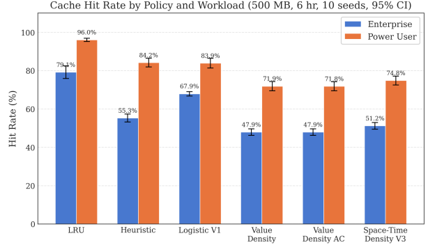
Figure 1: Cache hit rate by policy and workload with 95% CI error bars across 10 seeds. LRU dominates both constrained workloads.
