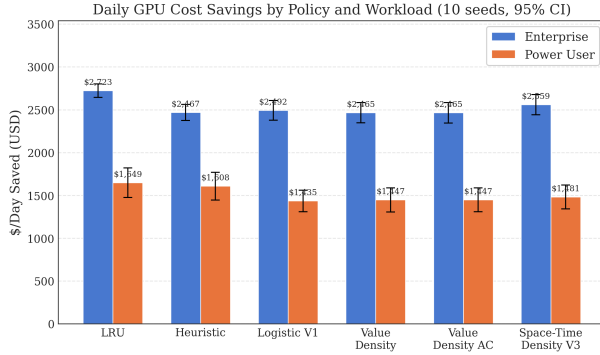
Figure 2: Daily GPU cost savings with 95% CIs. Note the compression of value gaps relative to hit-rate gaps on the power-user workload.
