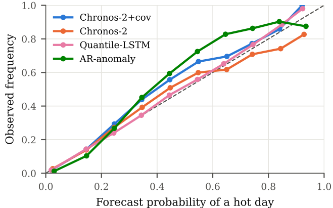
Reliability, hot day, leads 1-3
