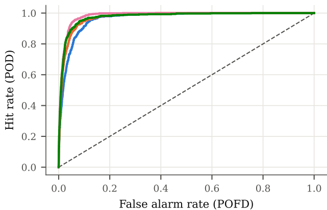
ROC, IMD heatwave, leads 1-3
