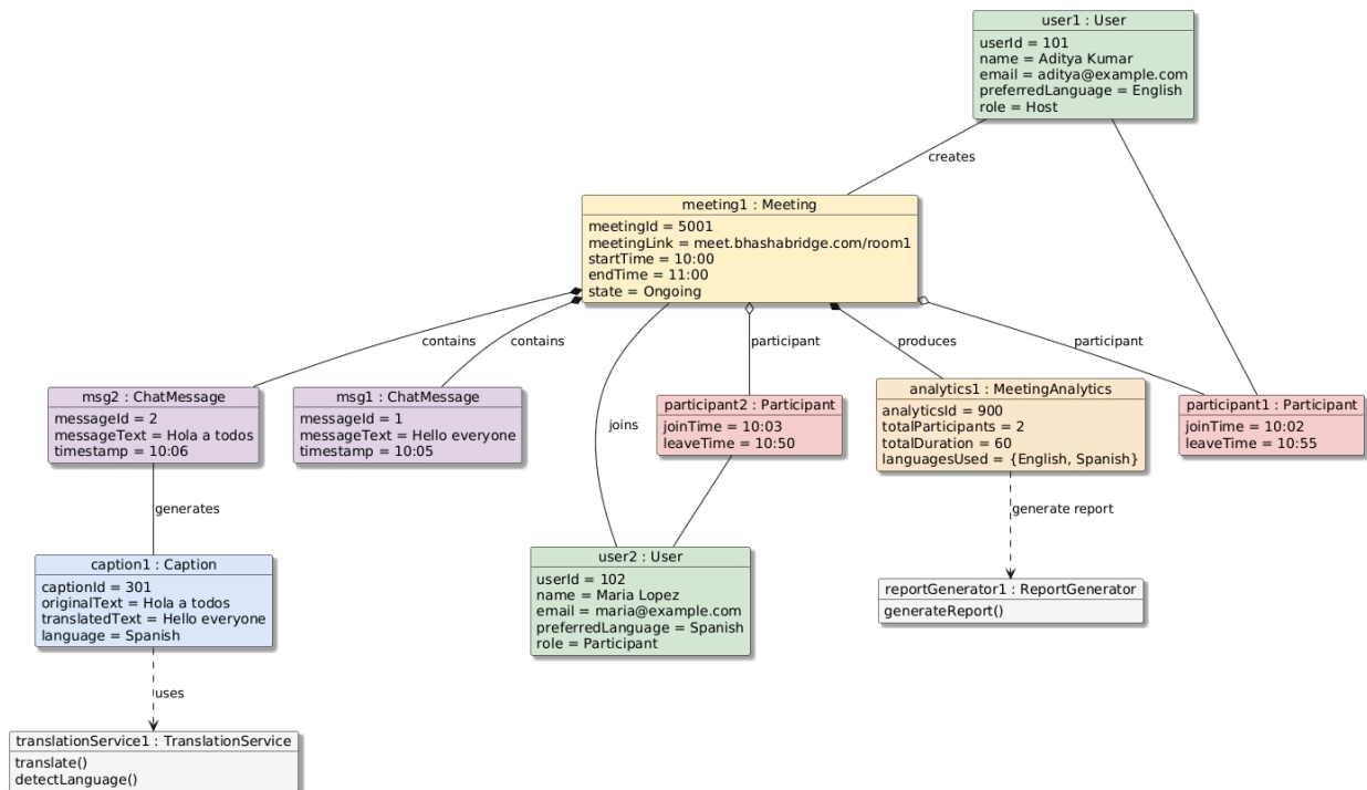
BhashaBridge Object Diagram - Runtime Snapshot
