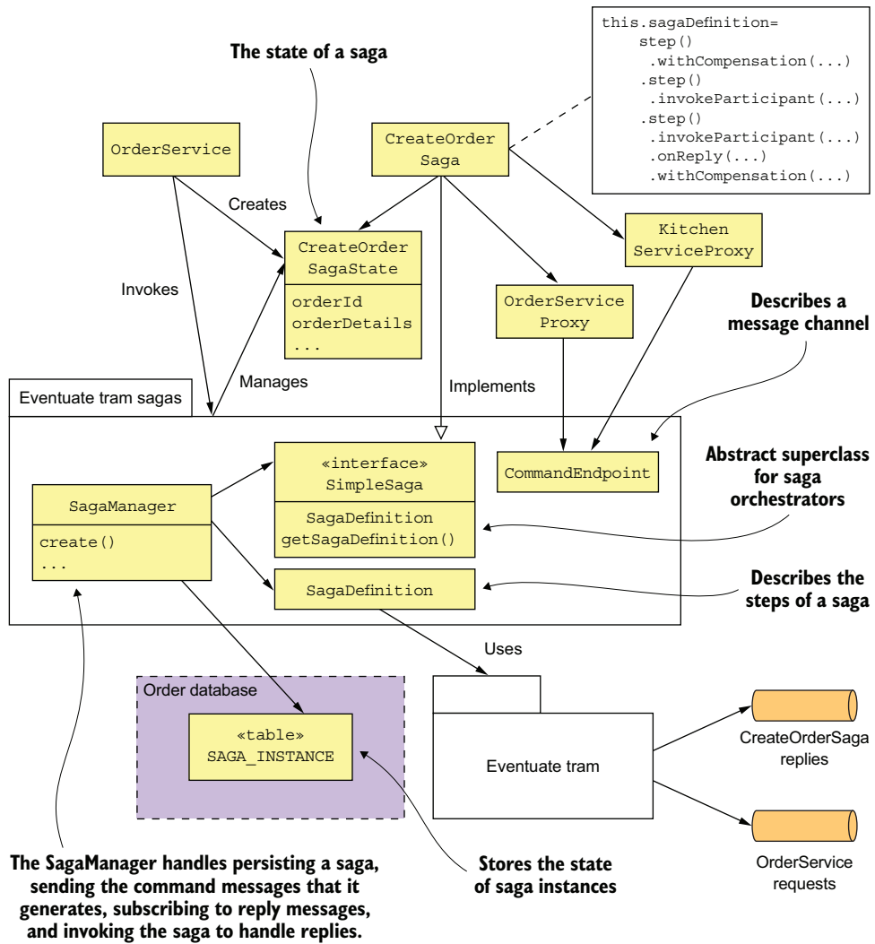
Figure 4.11 The OrderService's sagas, such as Create Order Saga, are implemented using the Eventuate Tram Saga framework.
