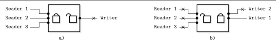
Figure 5-8. Readers-writer locks
