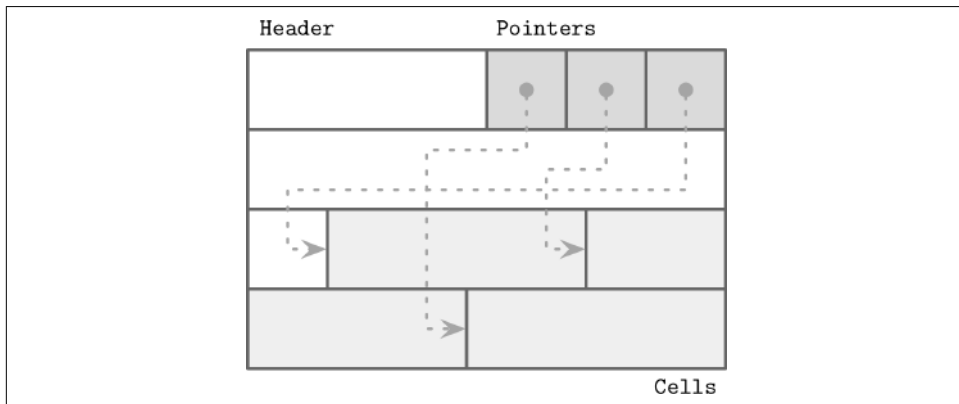
Figure 3-5. Slotted page
