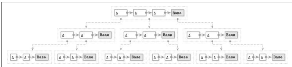
Figure 6-7. Bw-Tree. Dotted lines represent virtual links between the nodes, resolved using the mapping table. Solid lines represent actual data pointers between the nodes.
