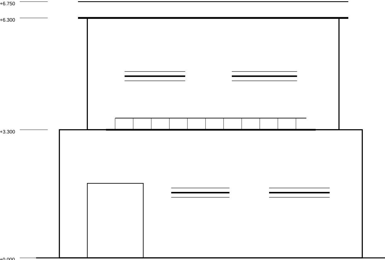
FRONT ELEVATION
