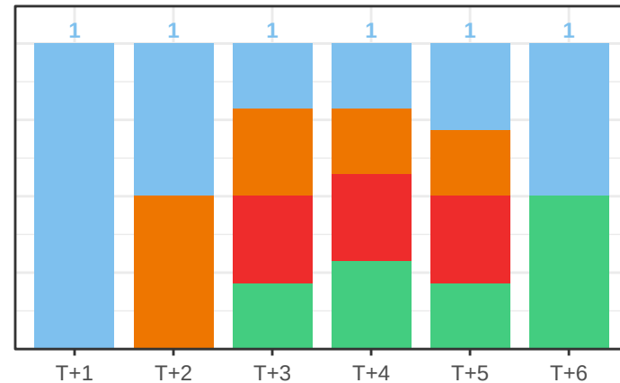
Conformal Prediction + 0
