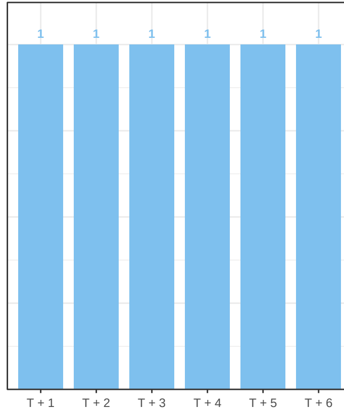
Likelihood-Based Prediction
