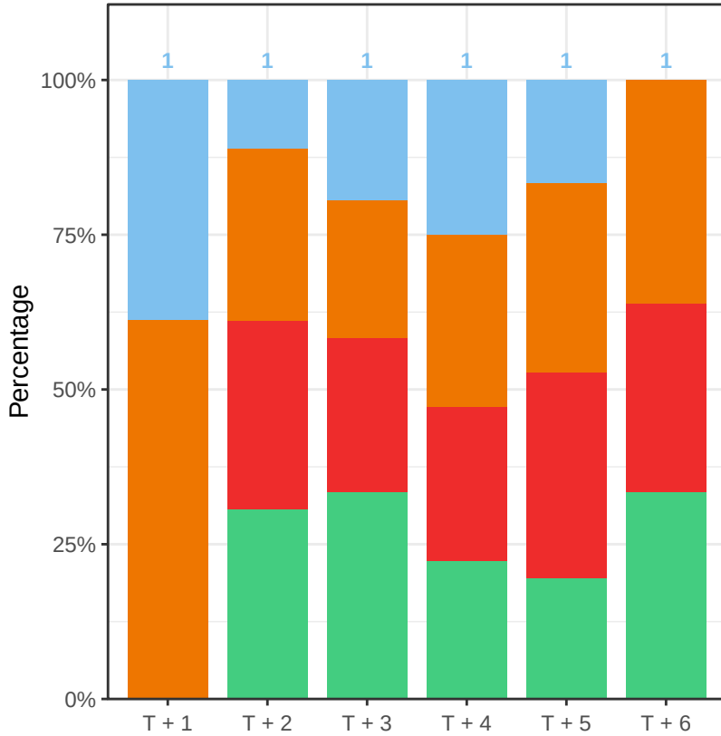
Conformal Prediction
