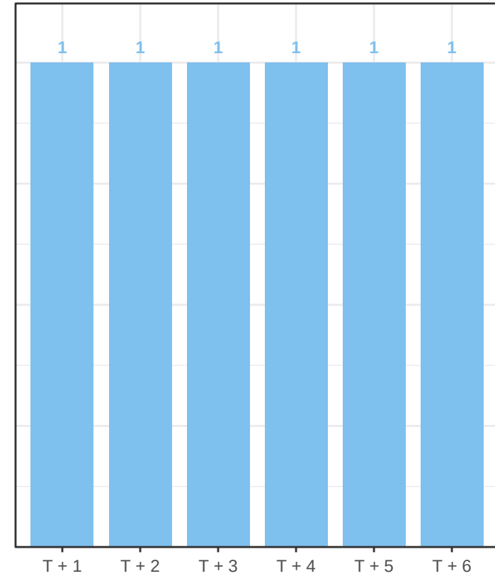
Conformal Prediction + 0
