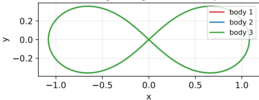
Validated figure-eight orbit (one period)
