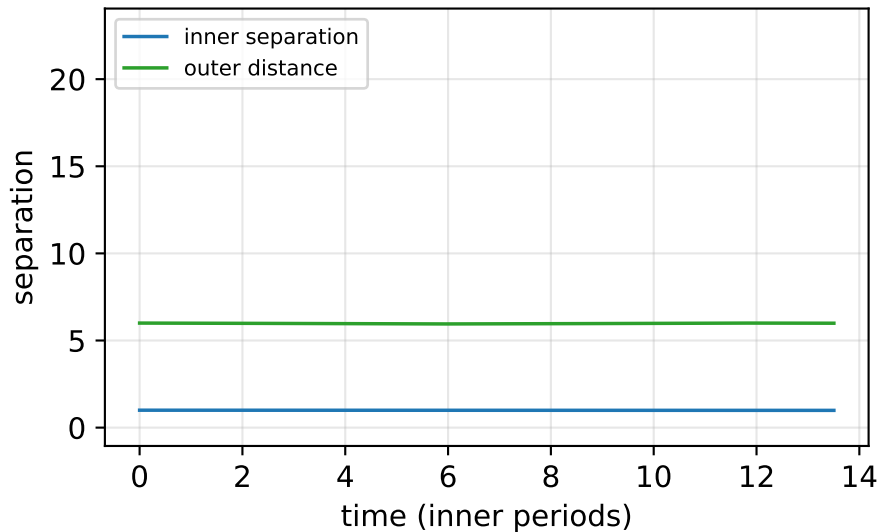
stable ( a_{\text{out}}/a_{\text{in}} = 6.0 )
