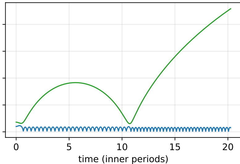
disrupted ( a_{\text{out}}/a_{\text{in}} = 1.8 )
