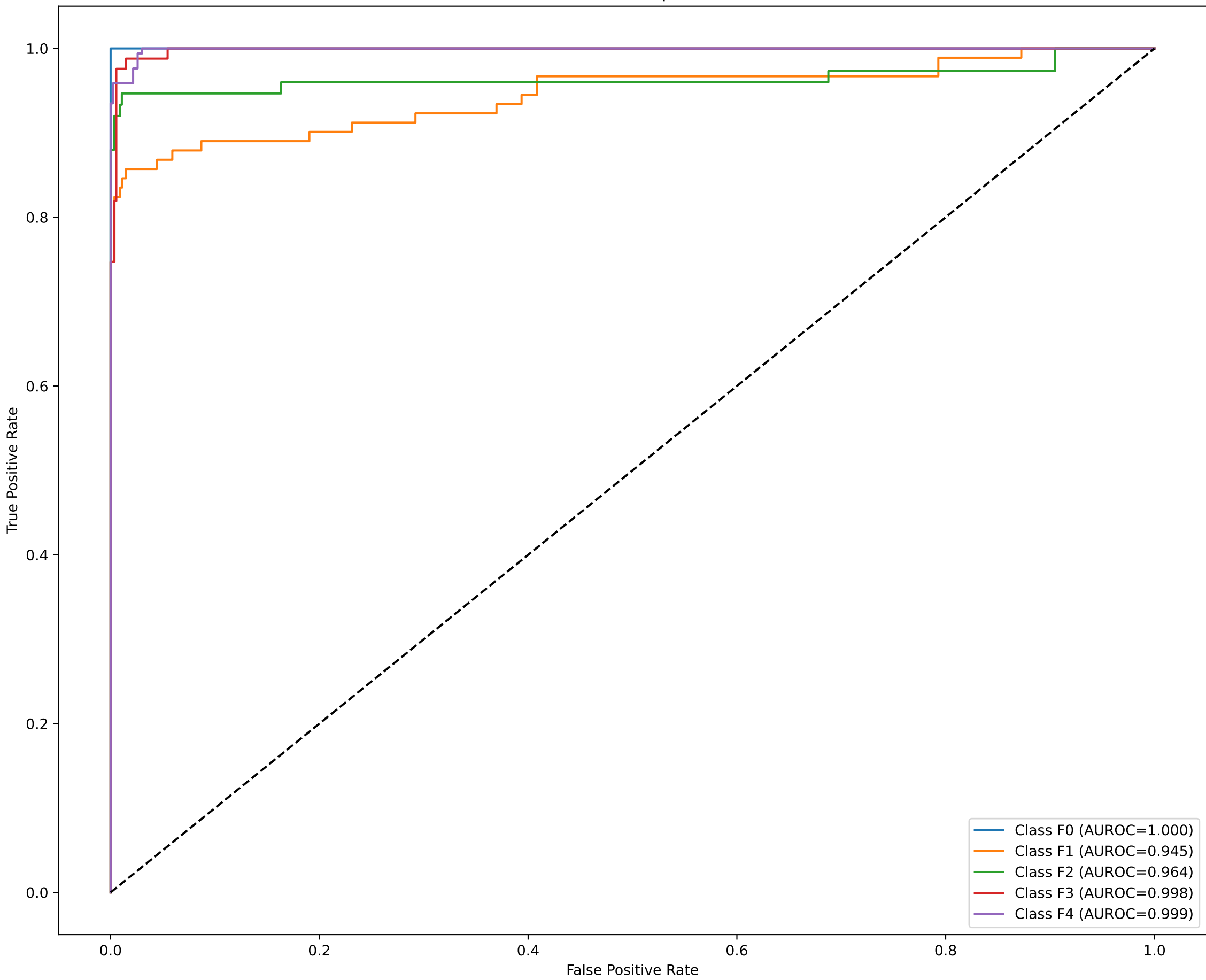
ROC Curve - Supervised
