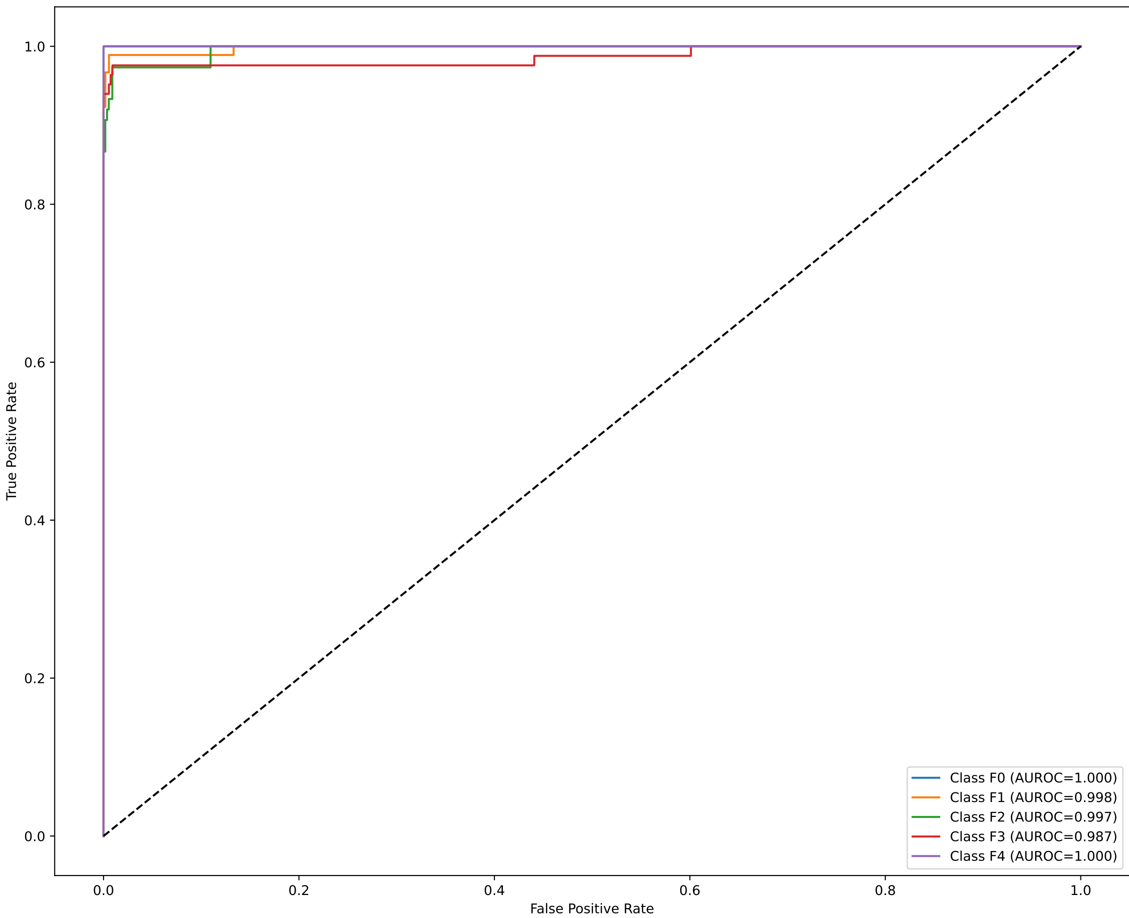
ROC Curve - Contrastive - 8 bit
