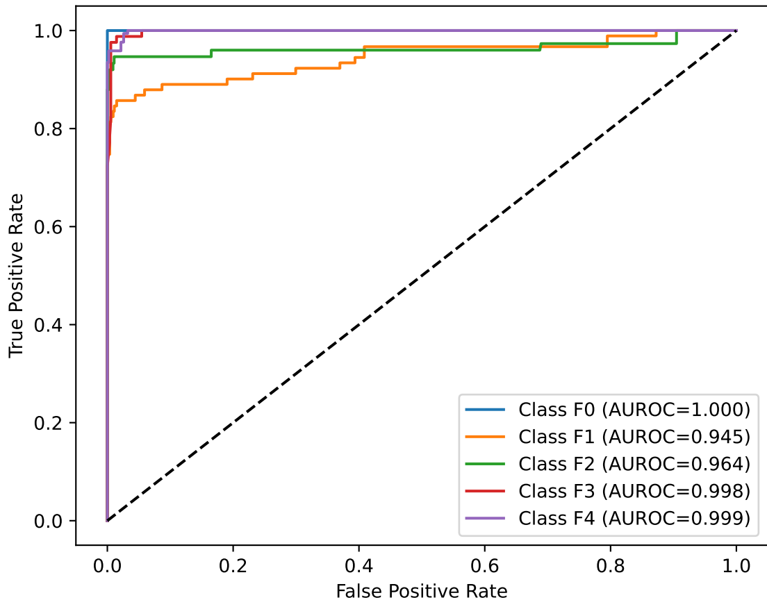
ROC Curve - Supervised - 16 bit
