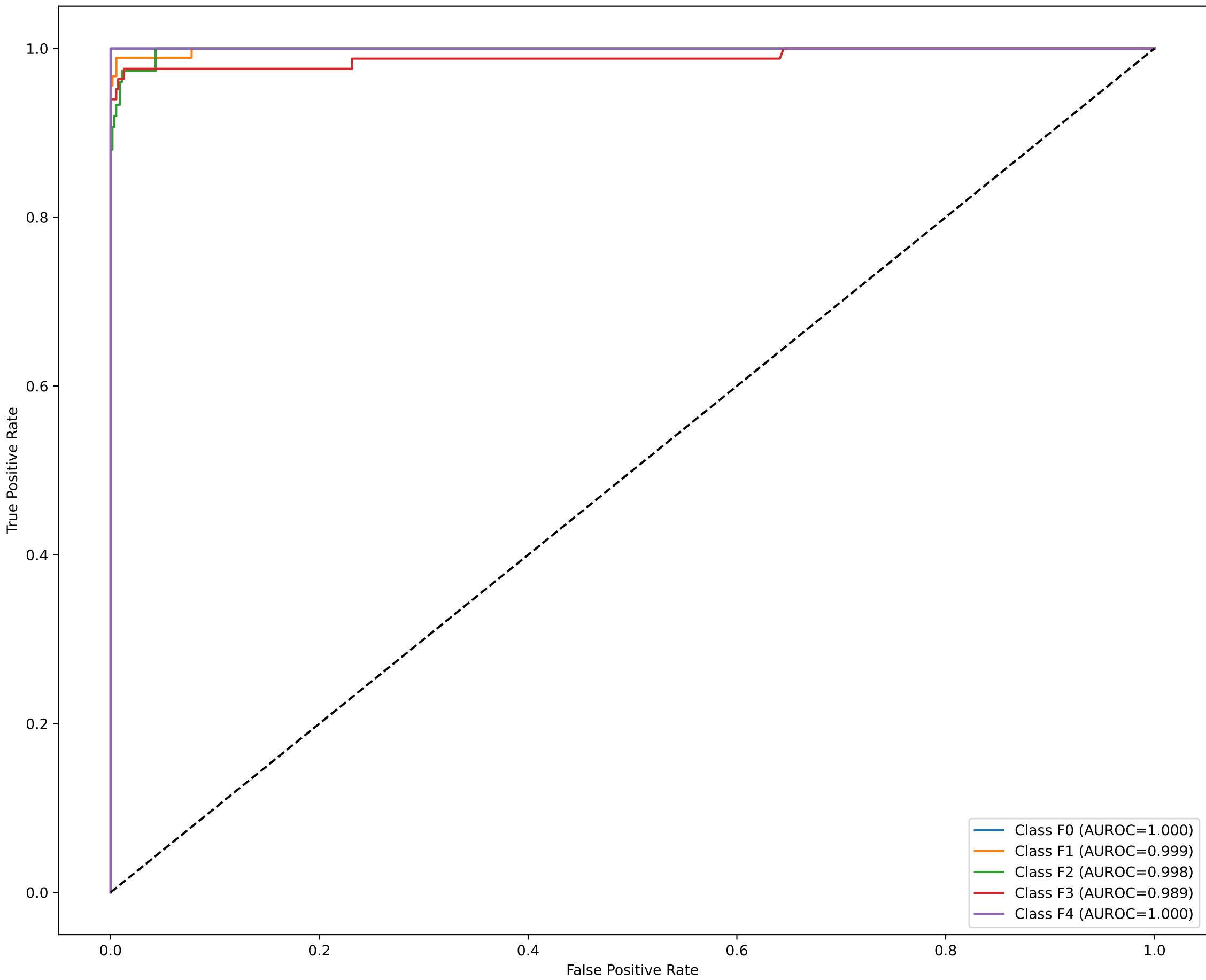
ROC Curve - Contrastive - 16 bit
