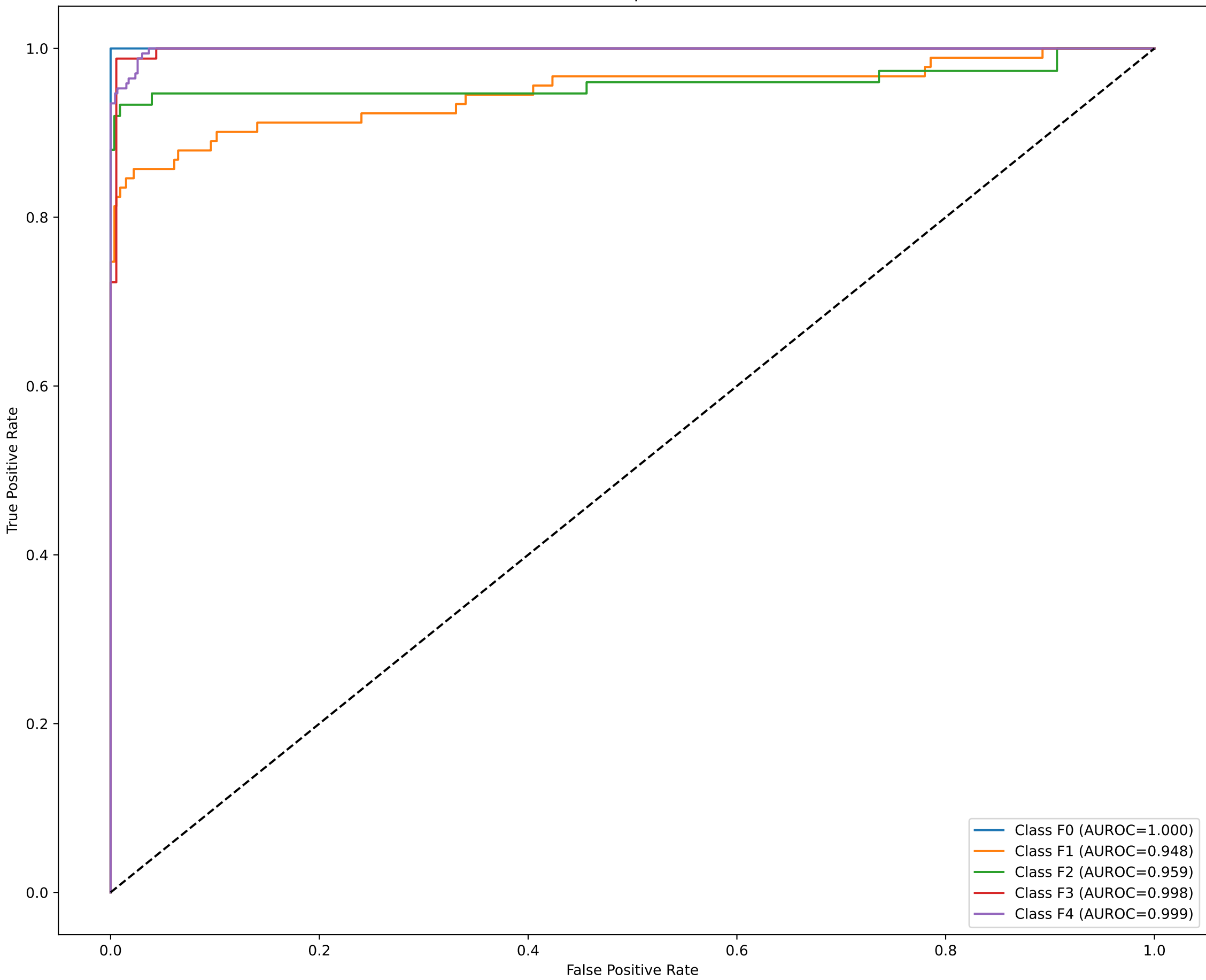
ROC Curve - Supervised - 8 bit
