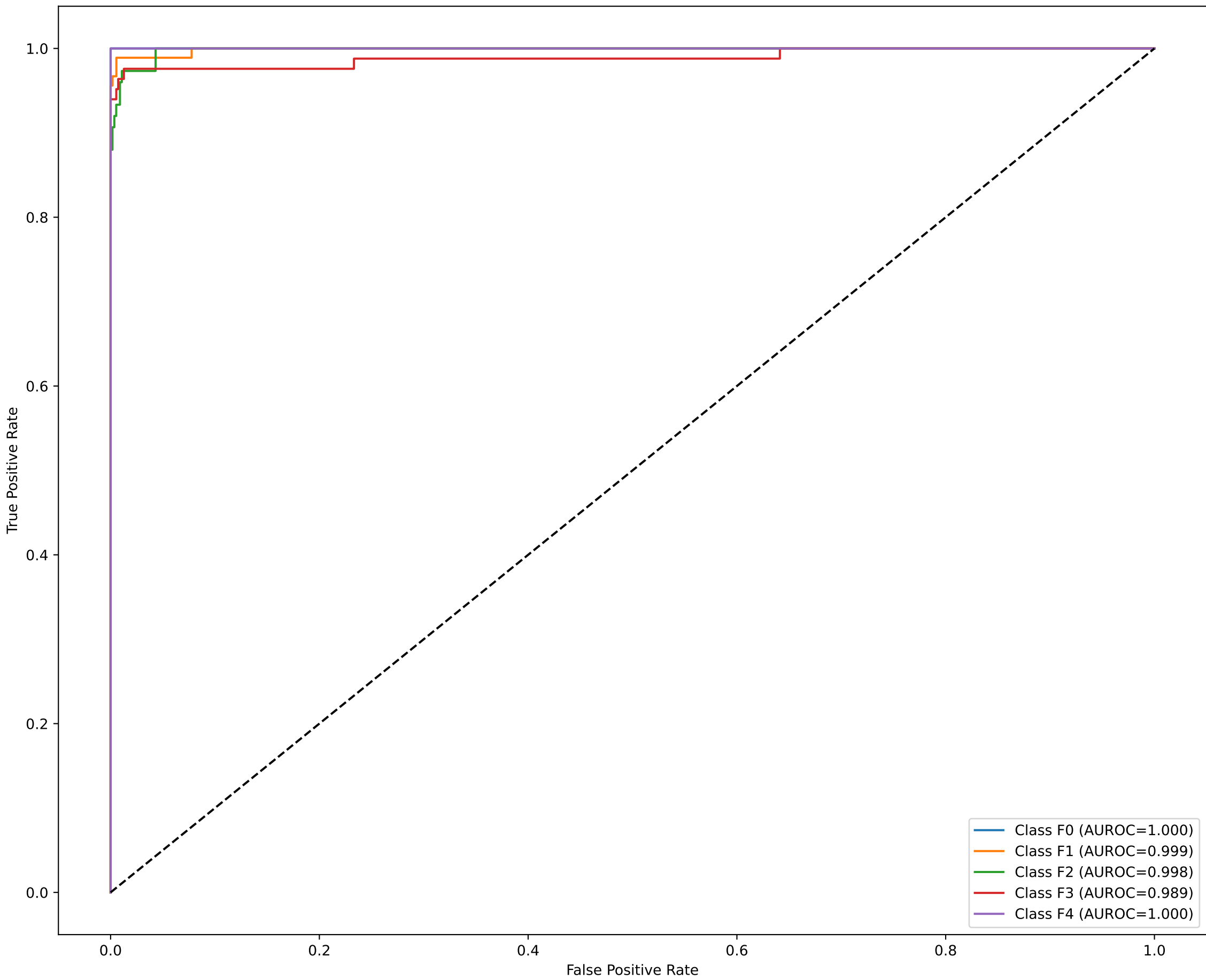
ROC Curve - Contrastive
