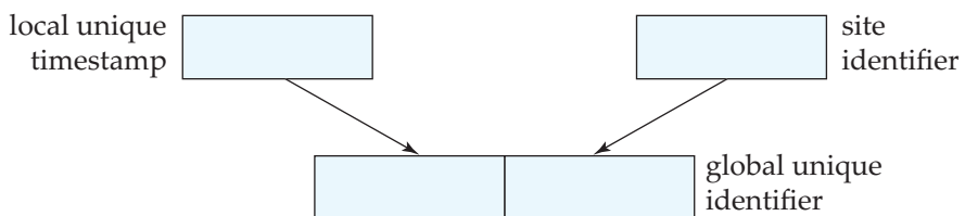
Figure 19.3 Generation of unique timestamps.
