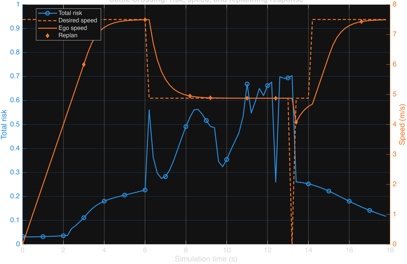
Cattle Crossing: risk, speed, and replanning response
