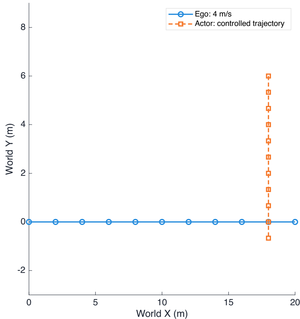
Farther collision course Distance 18.974 m | CPA 0.00 m at 4.5 s ACARG risk 0.412 | Without CPA 0.117
