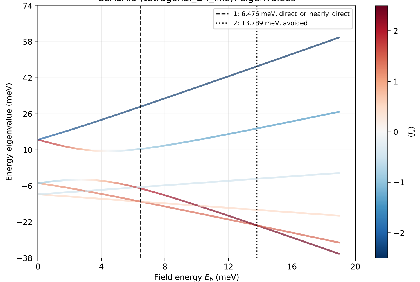
CeAuAl3 (tetragonal_D4_like): eigenvalues
