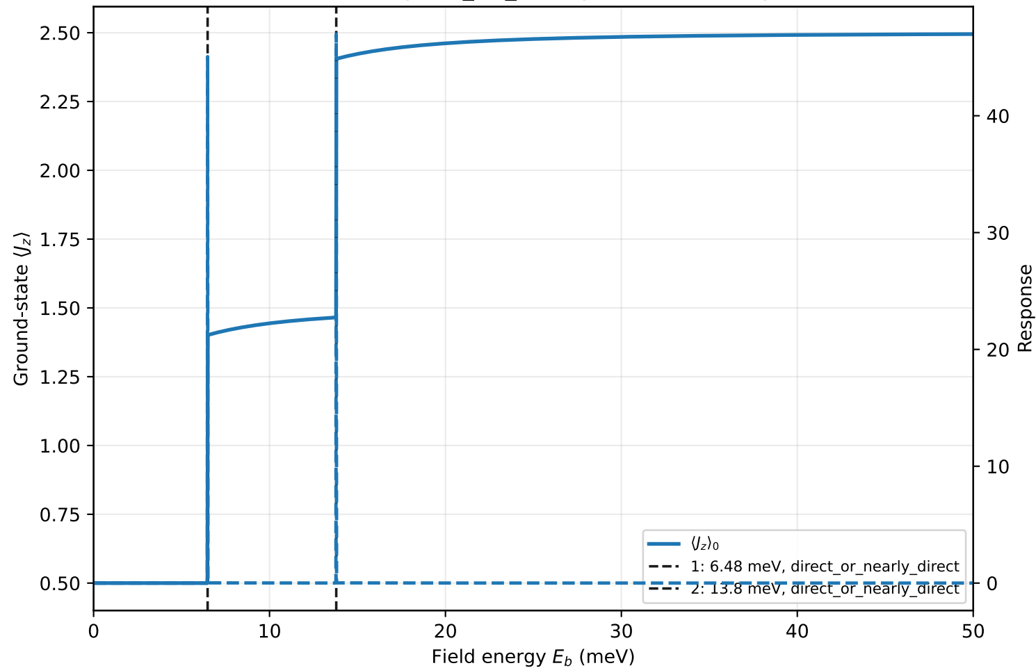
CeAuAl 3 (tetragonal_D4_like): ground-state response
