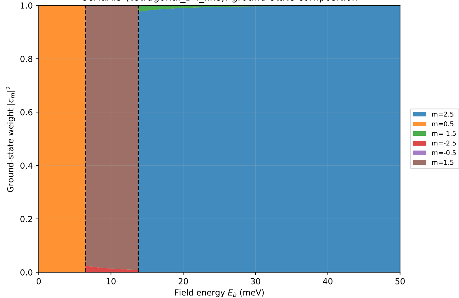
CeAuAl3 (tetragonal_D4_like): ground-state composition
