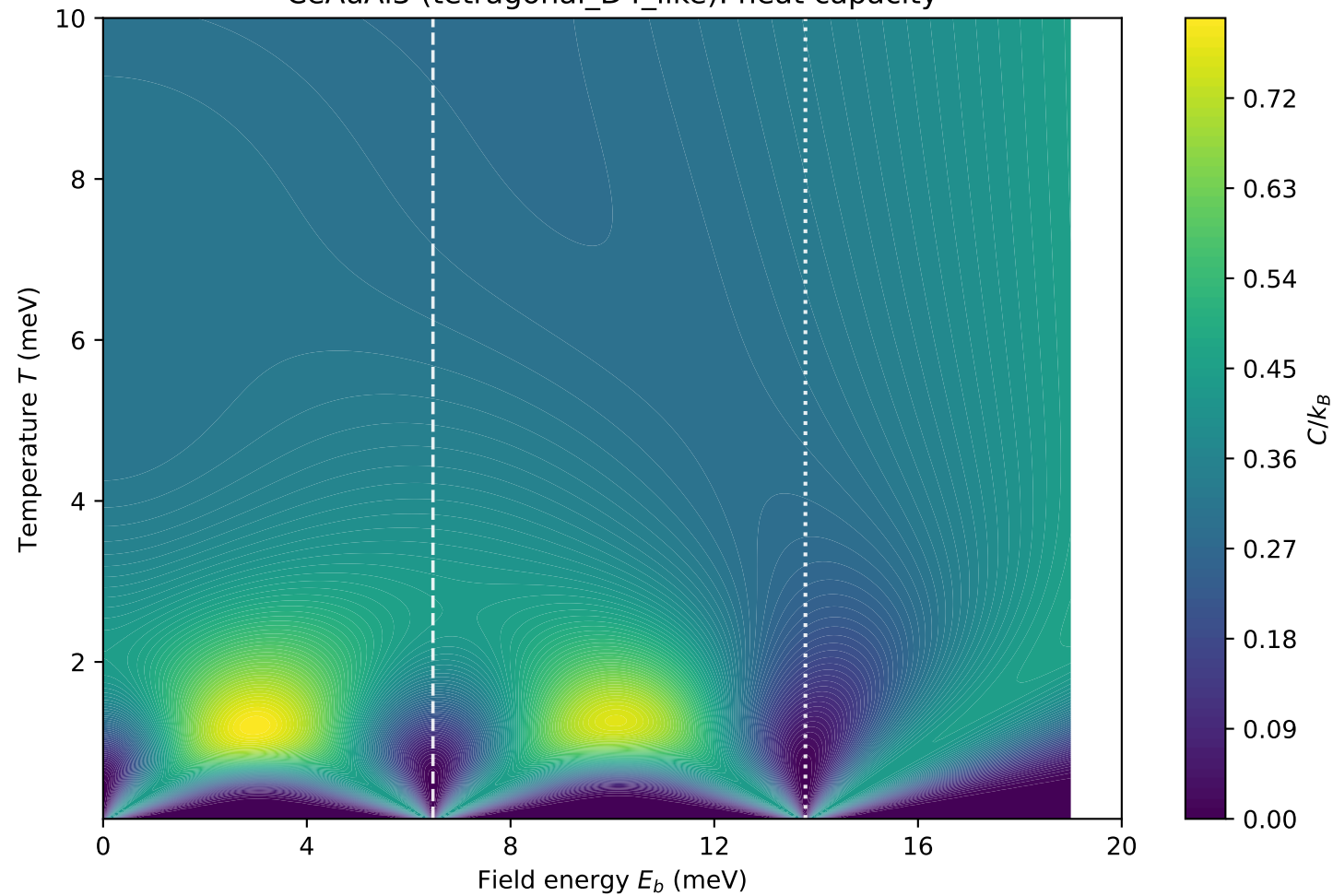
CeAuAl3 (tetragonal_D4_like): heat capacity
