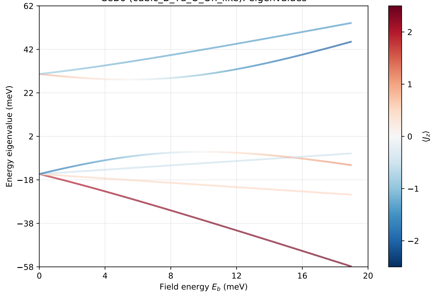
CeB6 (cubic_B_Td_O_Oh_like): eigenvalues
