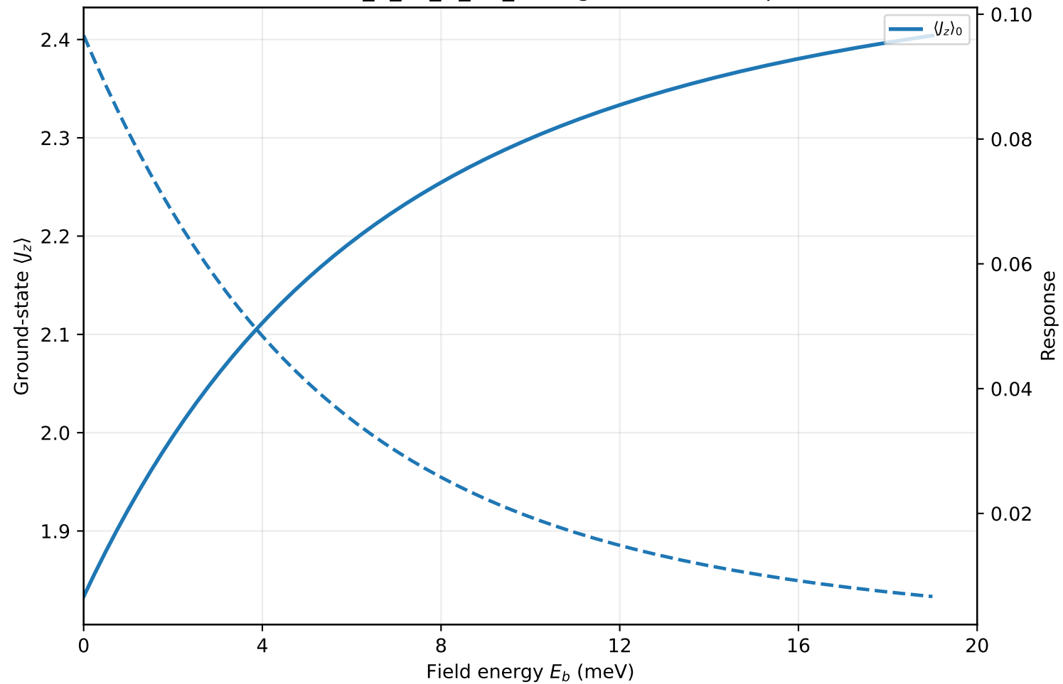
CeB6 (cubic_B_Td_O_Oh_like): ground-state response
