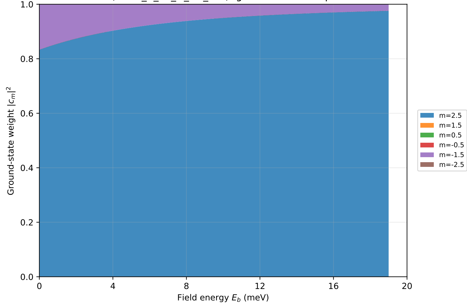
CeB6 (cubic_B_Td_O_Oh_like): ground-state composition
