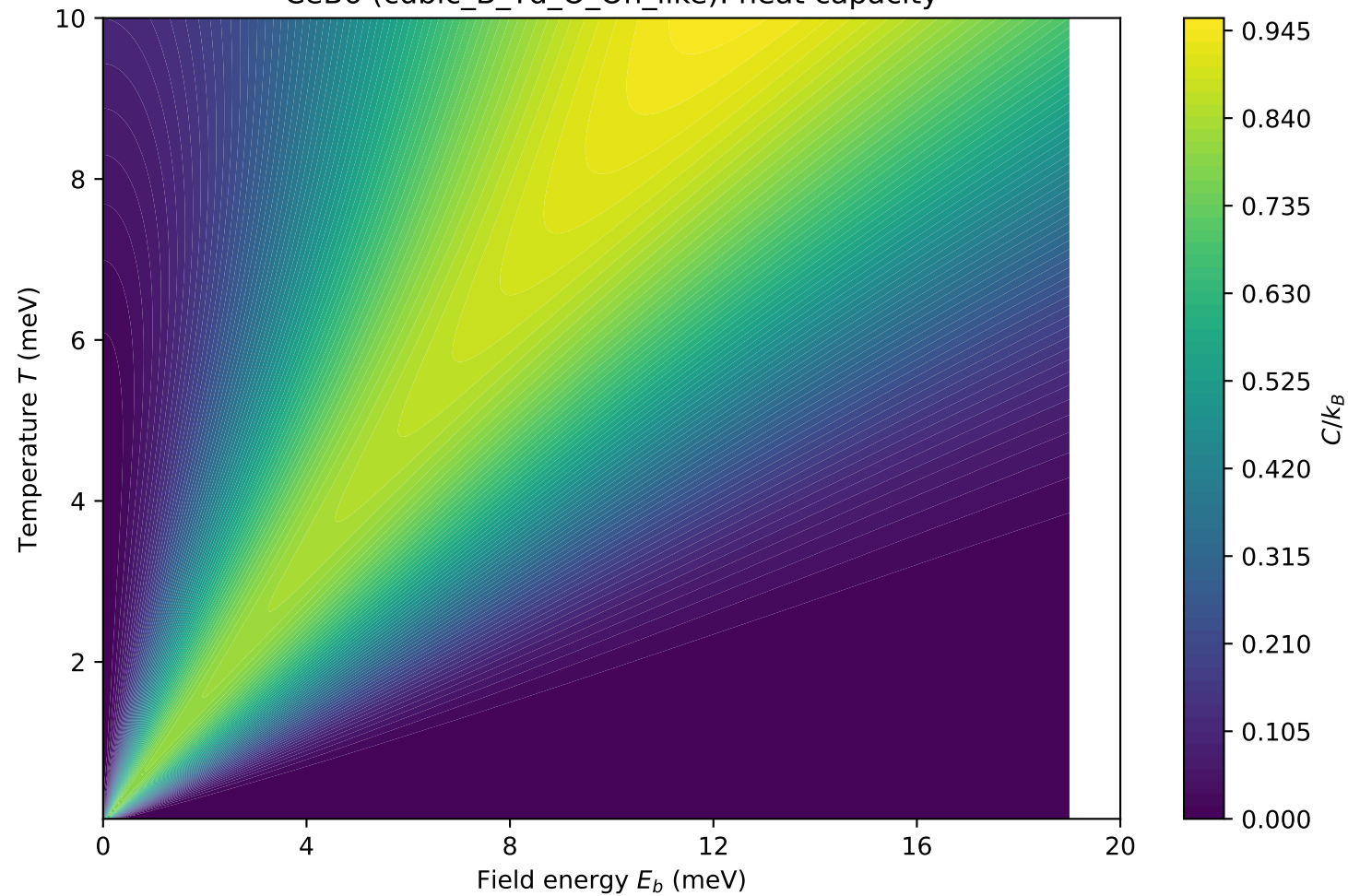
CeB6 (cubic_B_Td_O_Oh_like): heat capacity
