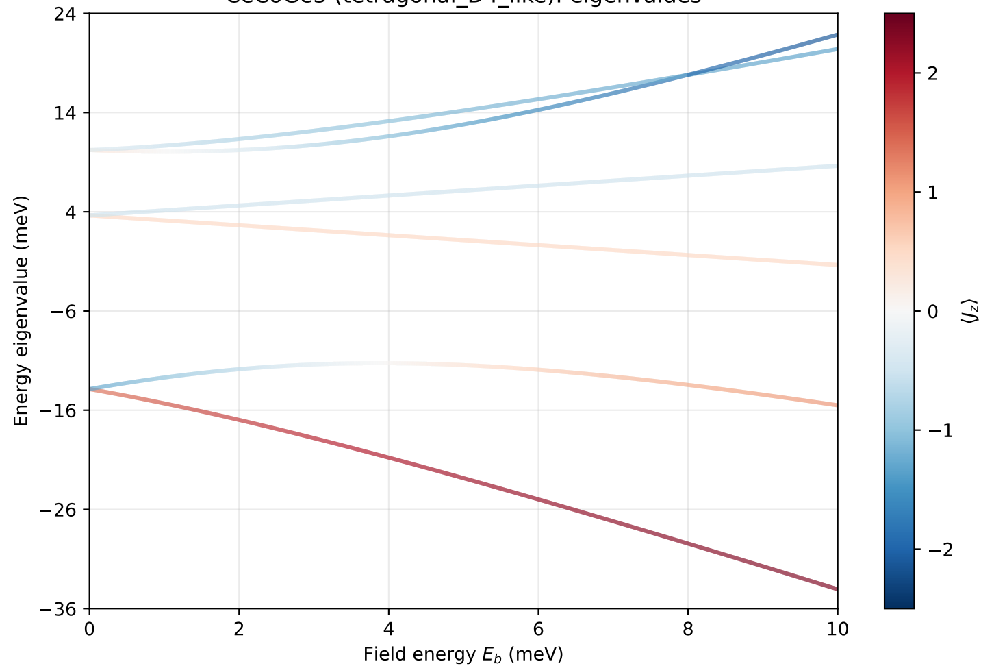
CeCoGe3 (tetragonal_D4_like): eigenvalues
