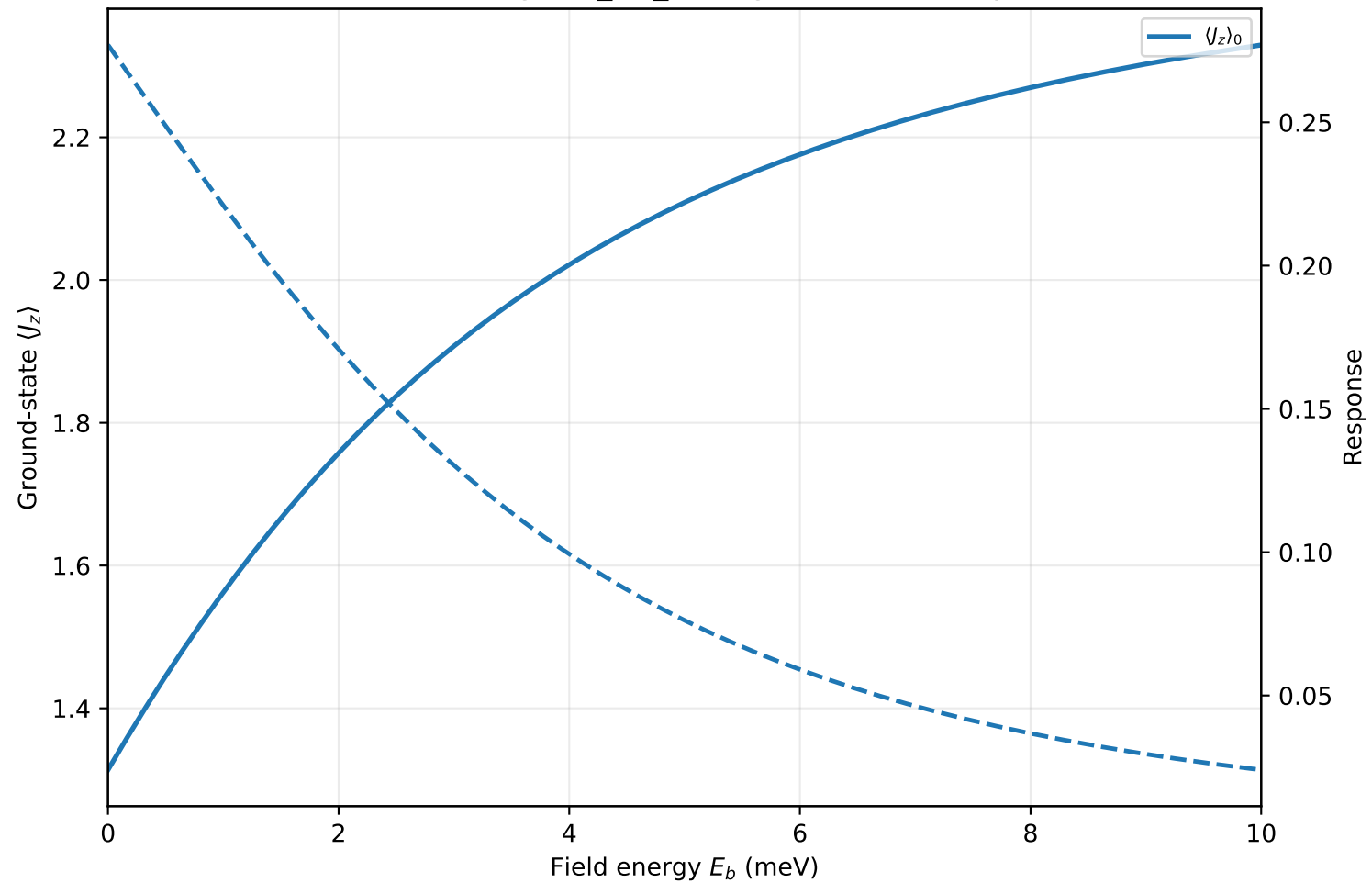
CeCoGe3 (tetragonal_D4_like): ground-state response
