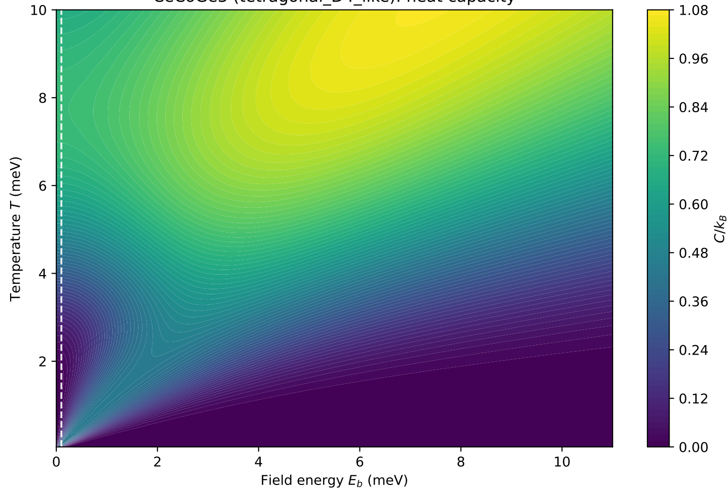
CeCoGe3 (tetragonal_D4_like): heat capacity
