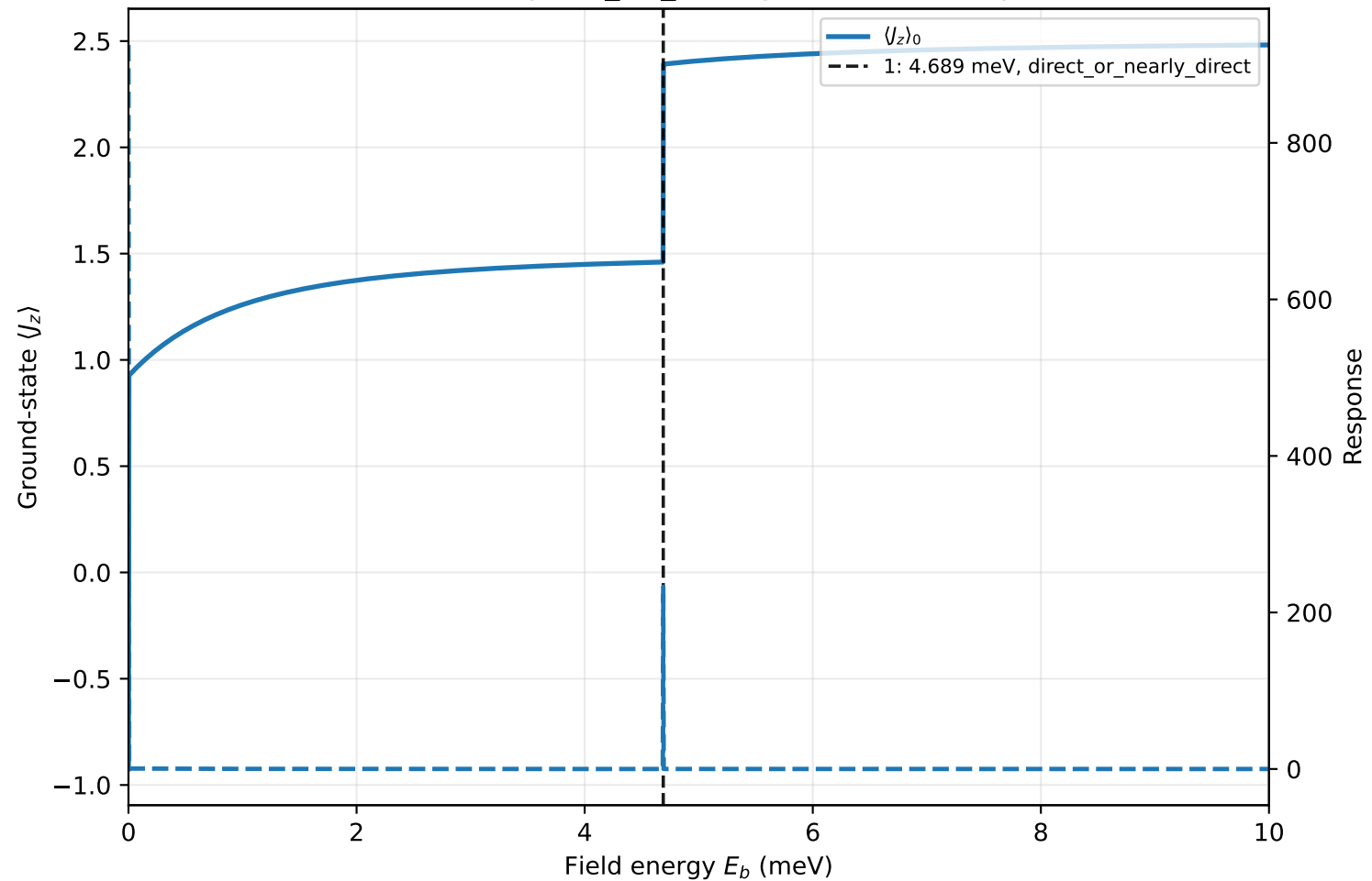
CeCoIn5 (tetragonal_D4_like): ground-state response
