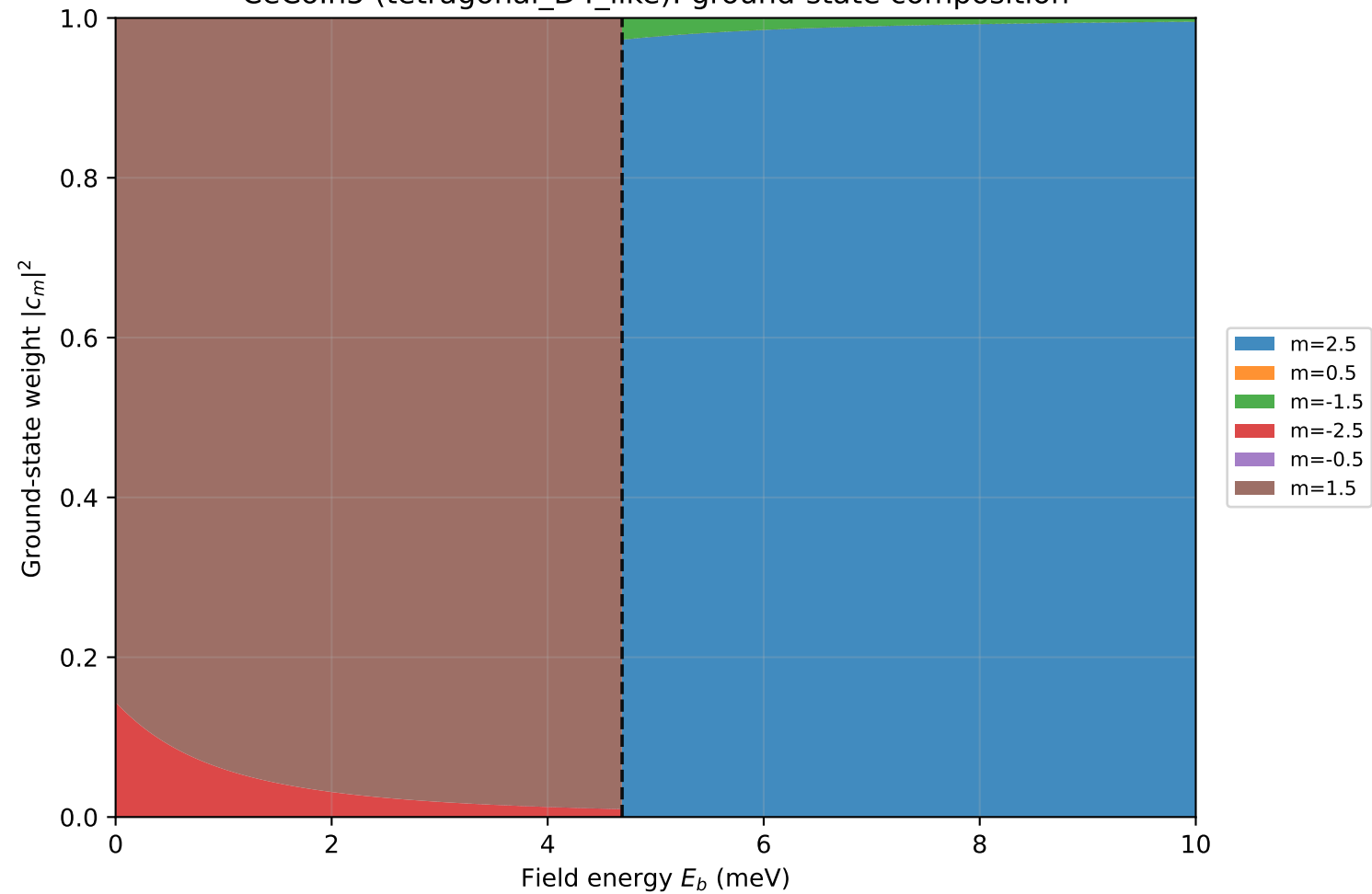
CeCoIn5 (tetragonal_D4_like): ground-state composition
