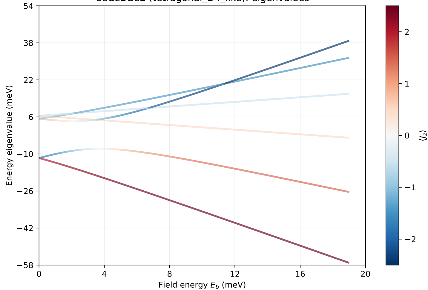
CeCu 2 Ge 2 (tetragonal_D4_like): eigenvalues
