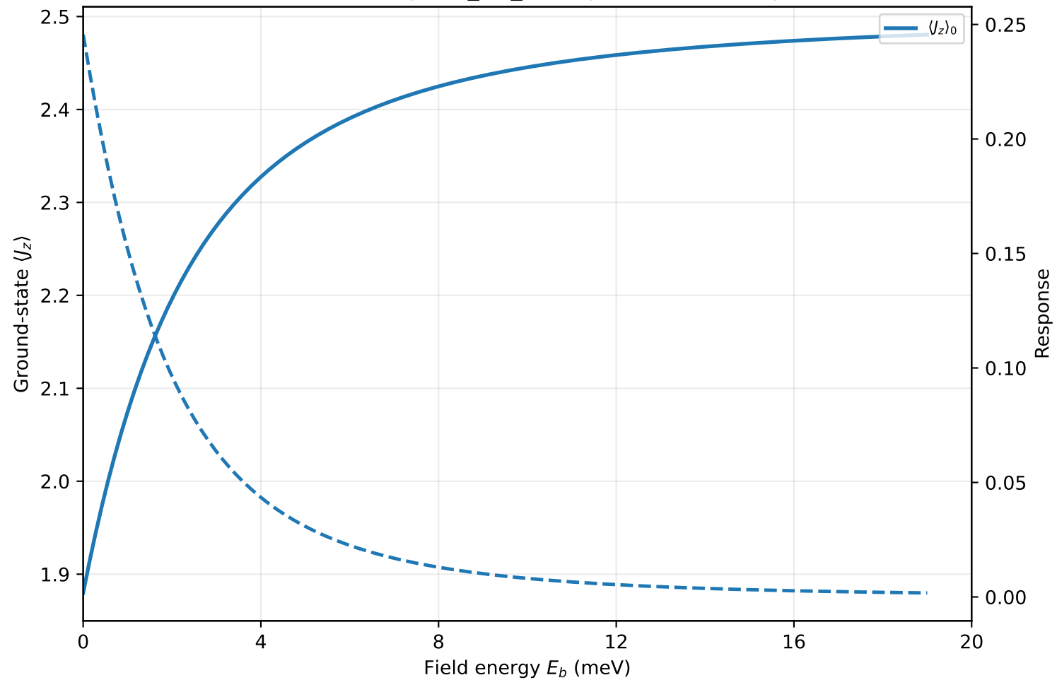
CeCu 2 Ge 2 (tetragonal_D4_like): ground-state response
